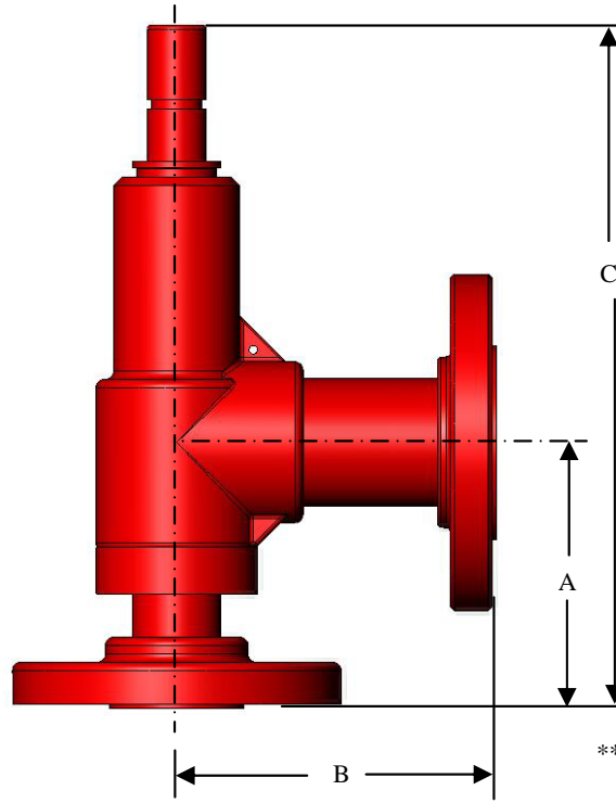
Flanged Configuration
