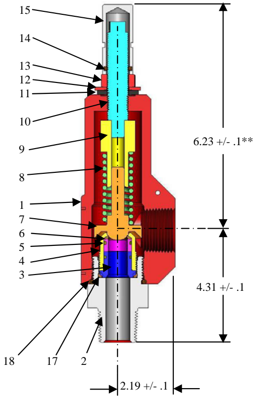
Threaded Configuration
