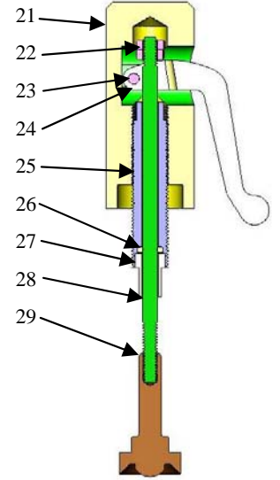
Lift Lever Components
