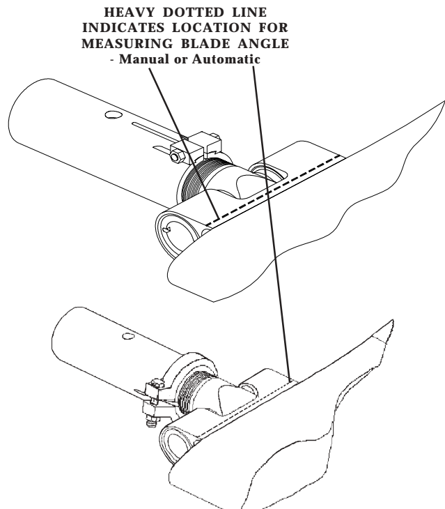
CLASS 10000 AUTOMATIC HUB DETAIL NOTE: CLAMP DIFFERENCES
